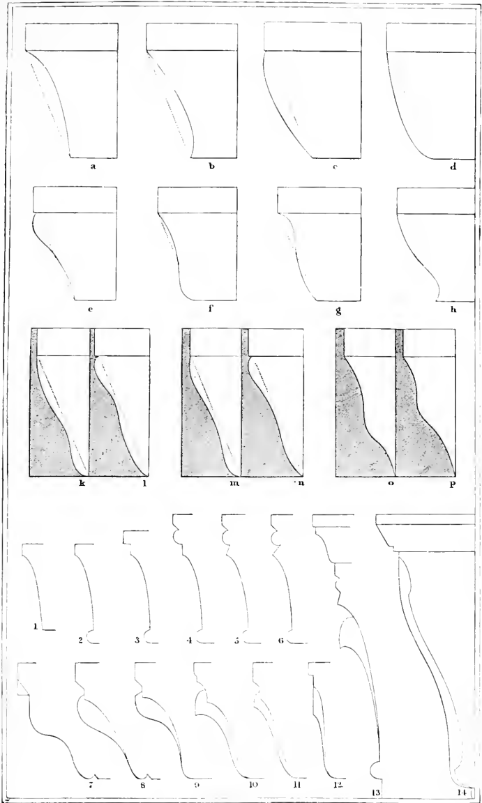
PLATE XV.—CORNICÉ PROFILES.
